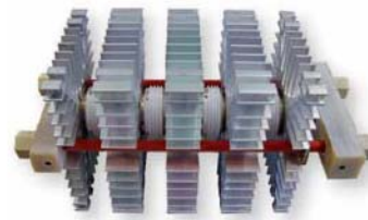
D Stack with 4 diodes connected in series using an insulated clamp system
