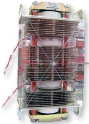
G Stack with two fast thyristors, air forced cooling system, four tie rod clamp
