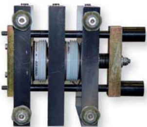
C Crow base stack
