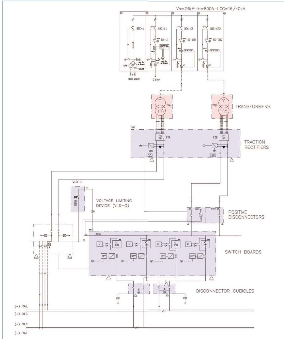
Typical schematic of a traction electrical substation
