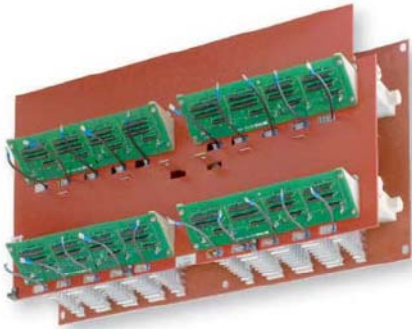
E Rectifier Monophase bridge, with snubber circuit board mounted on the top
