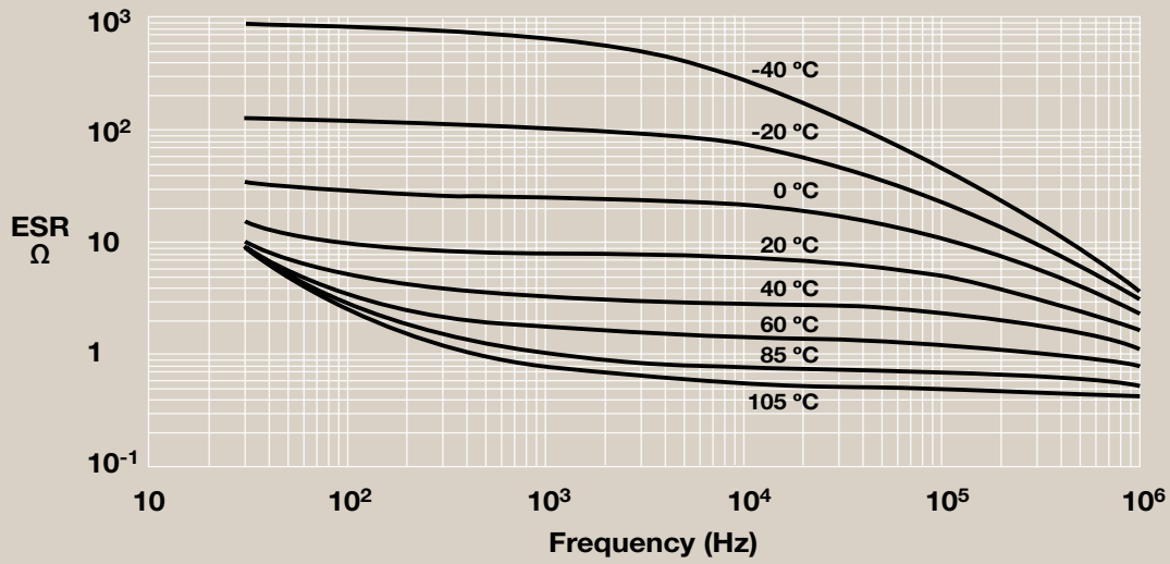
Figure 4a. Example of Aluminum Capacitor Characteristics (059 PLL-SI, 47 \mu\text{F}/400\text{ V} at 0 h)
