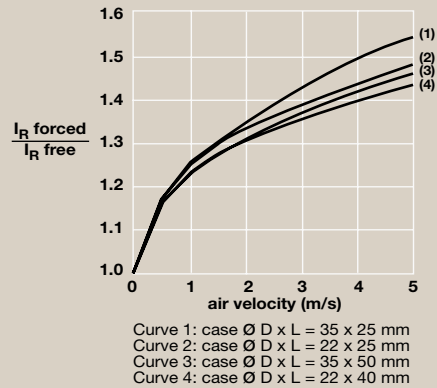
Figure 6. Transport of Heat from the Aluminum Capacitor to its Environment and the Effect of Airflow
