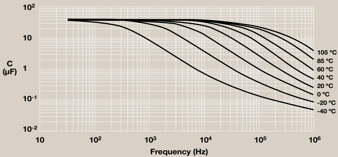
Figure 4b. Example of Aluminum Capacitor Characteristics (059 PLL-SI, 47 \mu\text{F}/400\text{ V} at 0 h)
