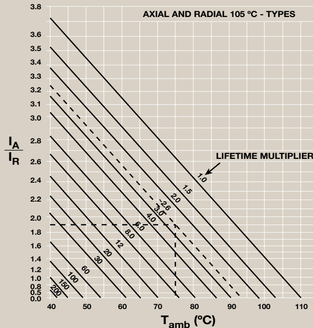
Figure 5. Example of a Lifetime Nomogram (This figure relates to Example 2)
