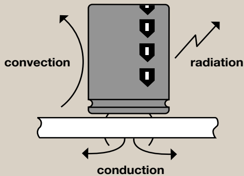
Figure 6. Transport of Heat from the Aluminum Capacitor to its Environment and the Effect of Airflow
