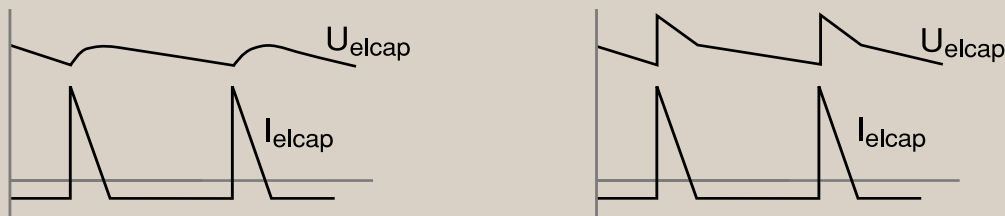
Figure 7. Voltage Ripple on Aluminum Capacitors without and with ESR
