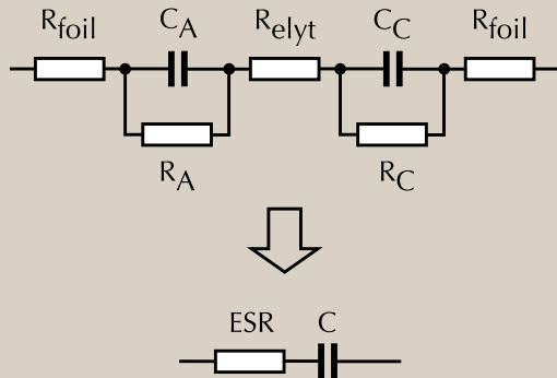
Figure 3. Equivalent AC Circuit
