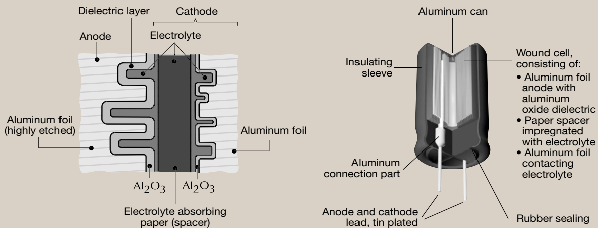
Figure 2. Basic Construction of Non-Solid Aluminum Capacitors
